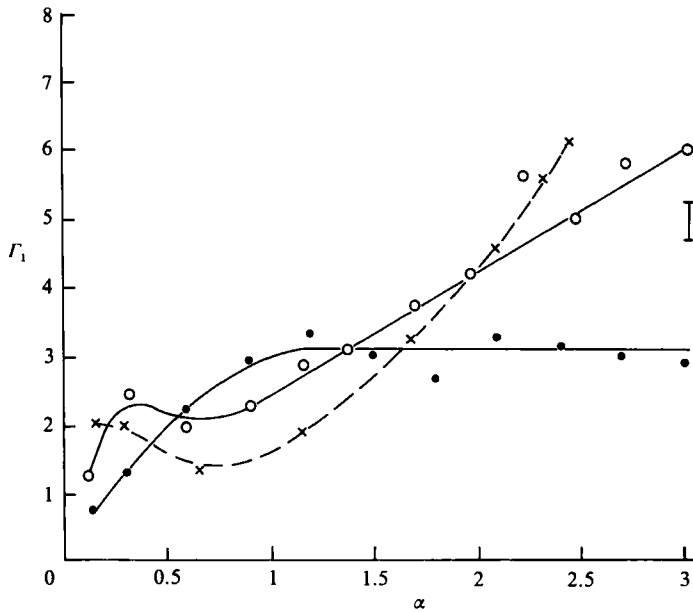
FIGURE 8. Dimensionless circulations, normalized by the mean angular velocity, for cases C3 (●—●), F3 (○—○) and results from Maxworthy's high- Re ( 1.3 \times 10^4 ) case (×—×). \Gamma_1 = \Gamma/\Omega c^2 .
